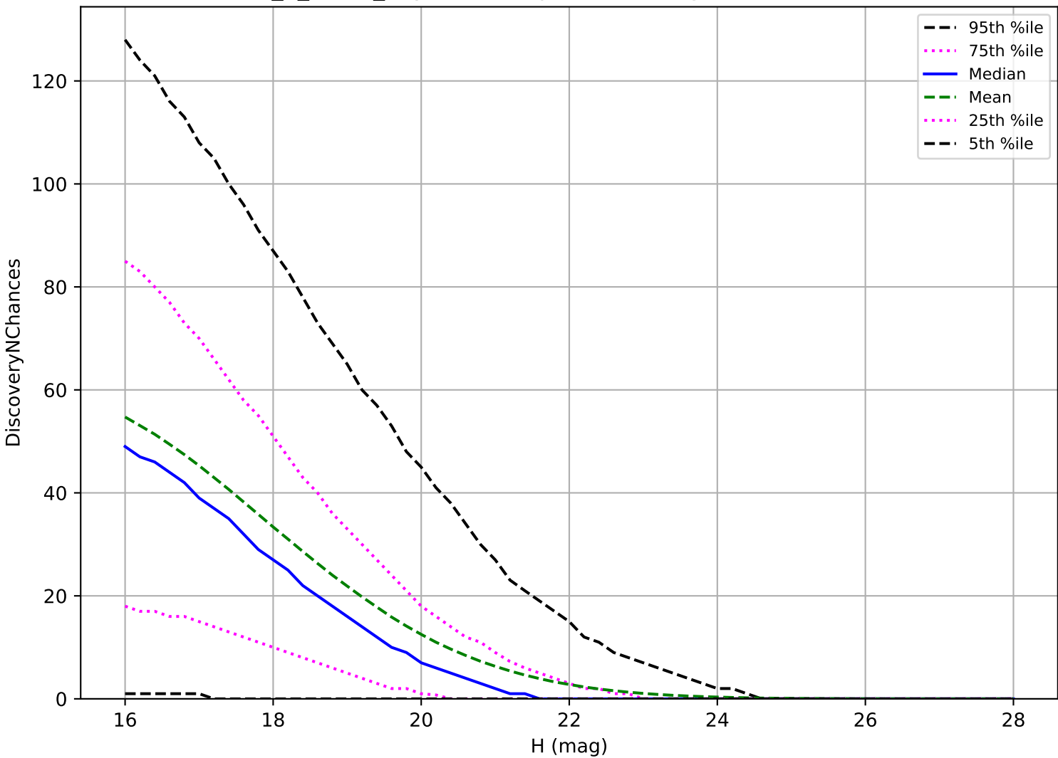
too_5_4v3.4_10yrs: PHA 3 pairs in 15 nights detection loss
