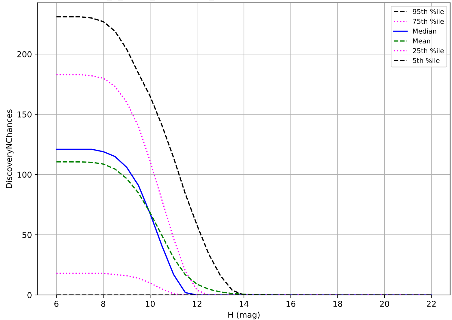
too_5_4v3.4_10yrs: OCC_r20 3 pairs in 15 nights detection loss
