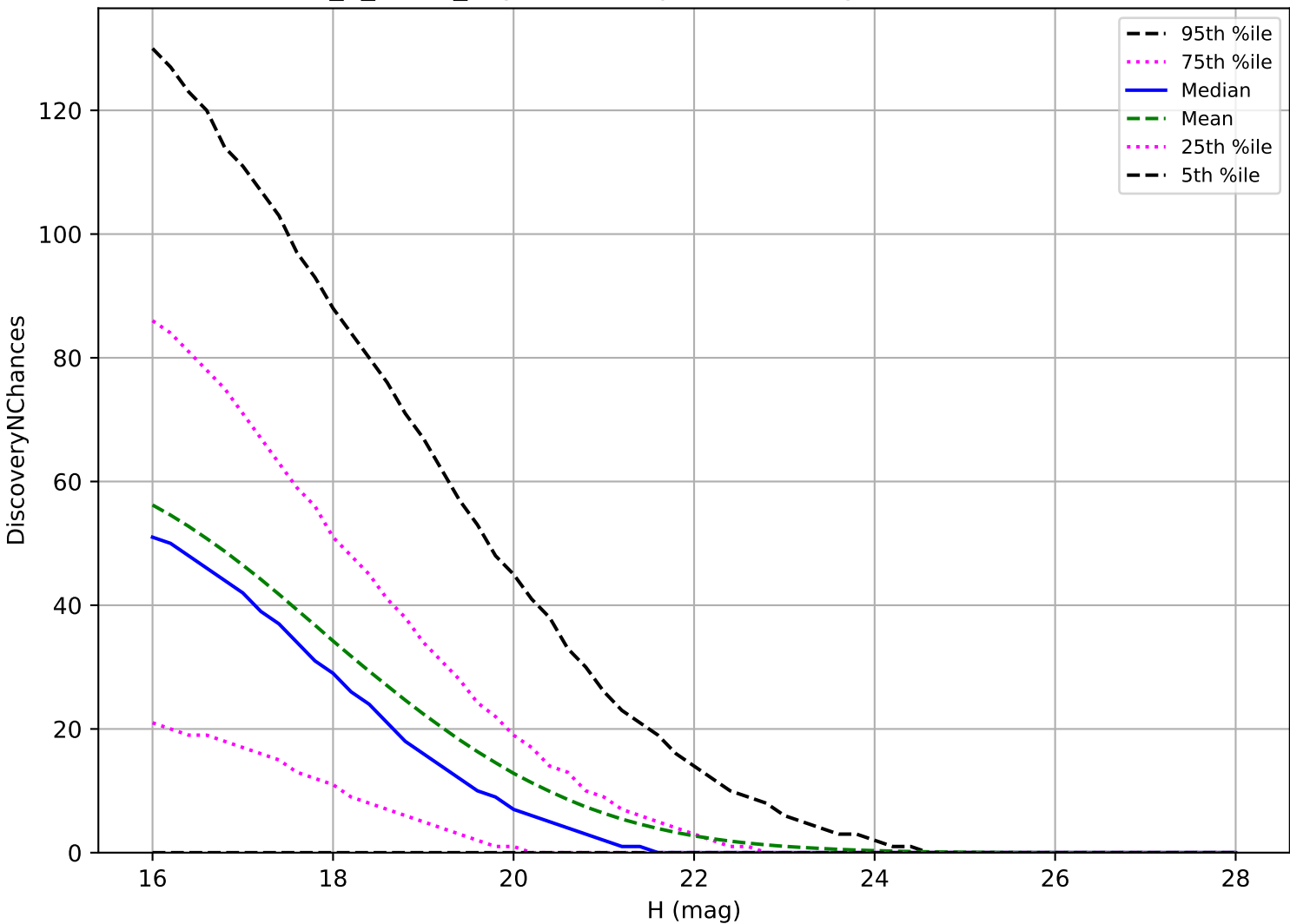
too_5_4v3.4_10yrs: NEO 3 pairs in 15 nights detection loss
