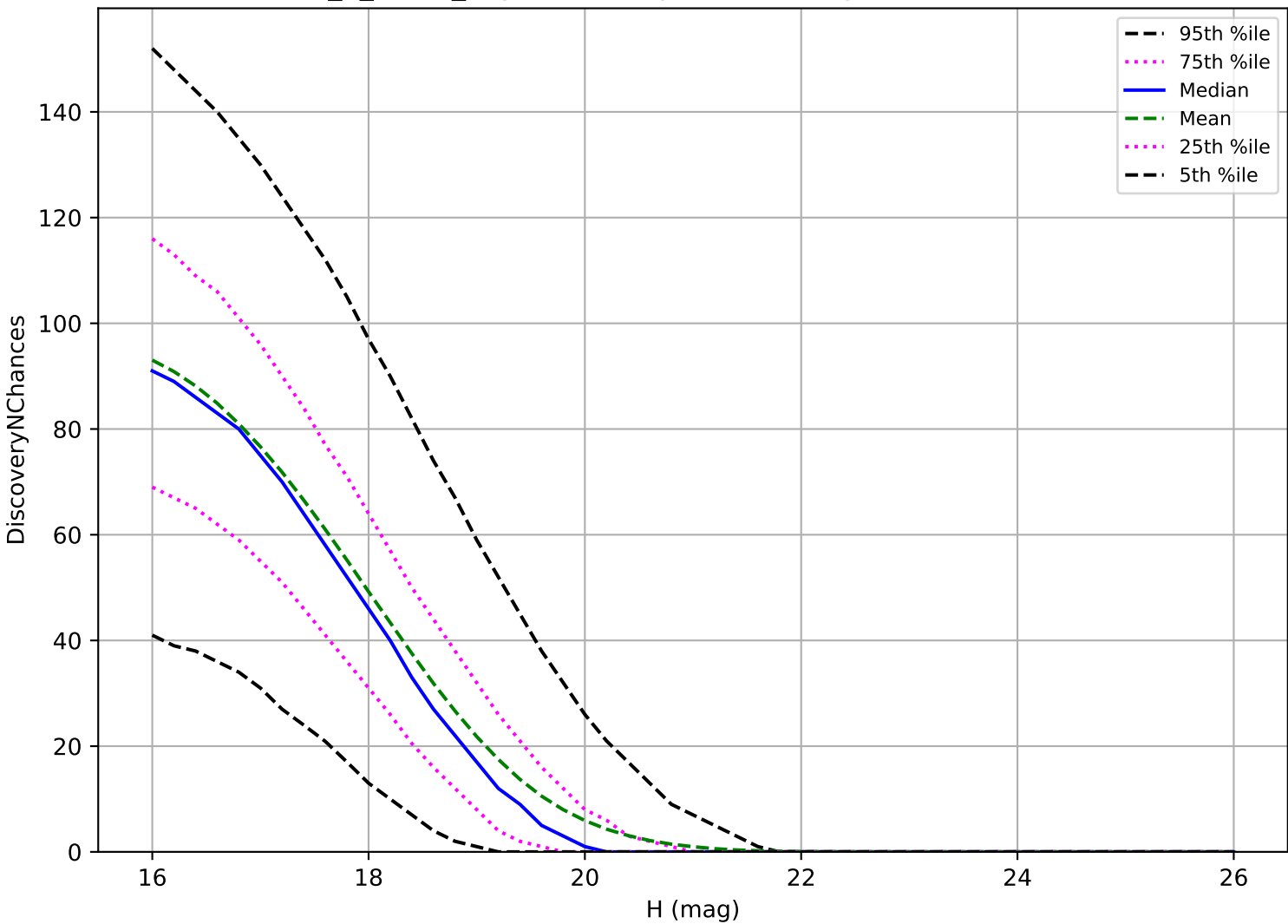
too_5_4v3.4_10yrs: MBA 3 pairs in 15 nights detection loss
