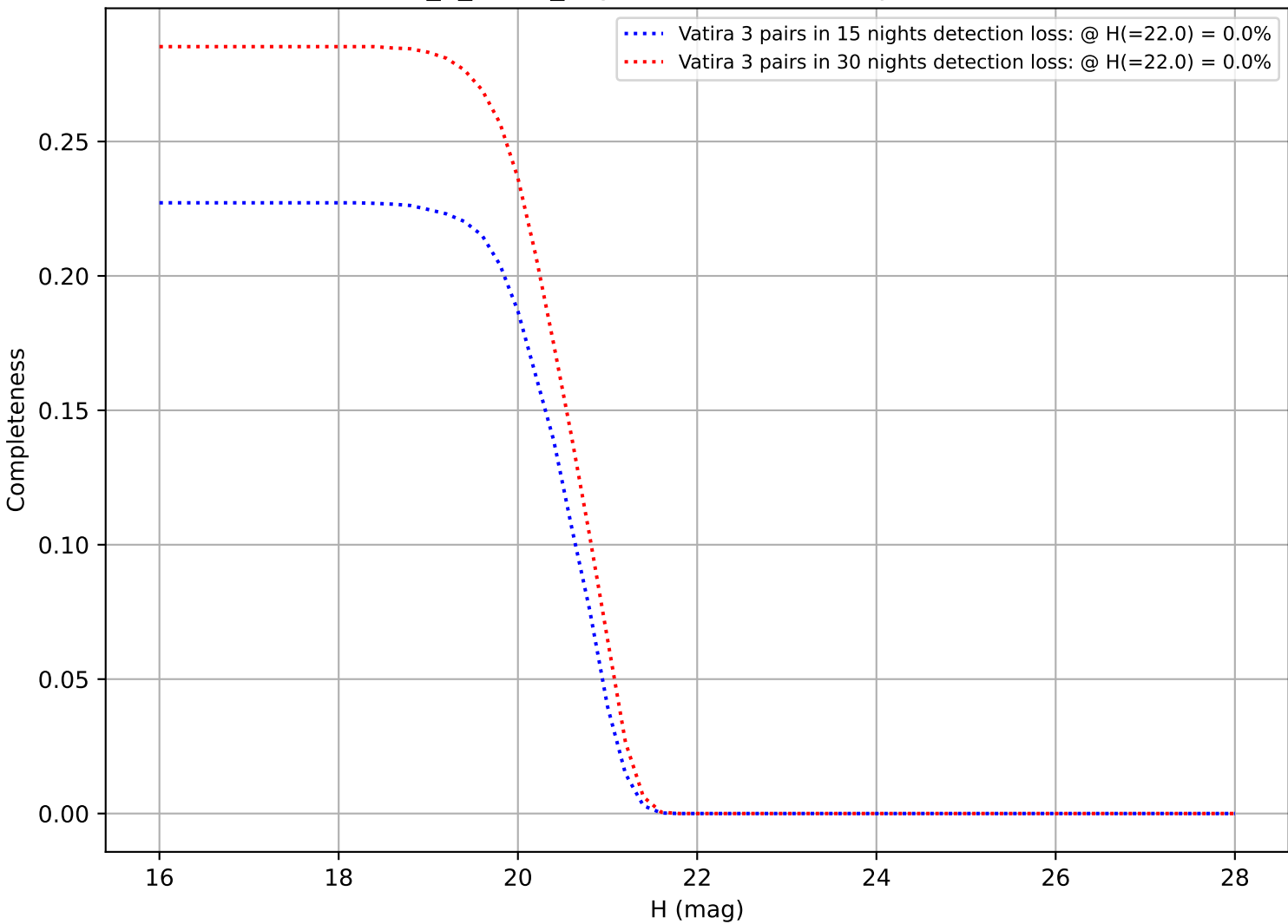
too_5_4v3.4_10yrs: DifferentialCompleteness
