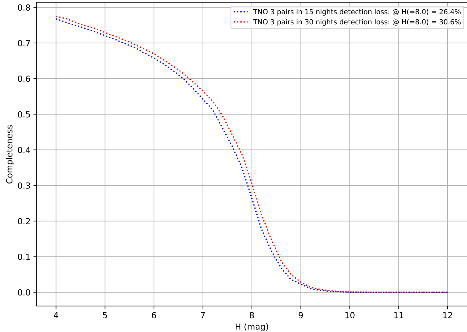
too_5_4v3.4_10yrs: DifferentialCompleteness
