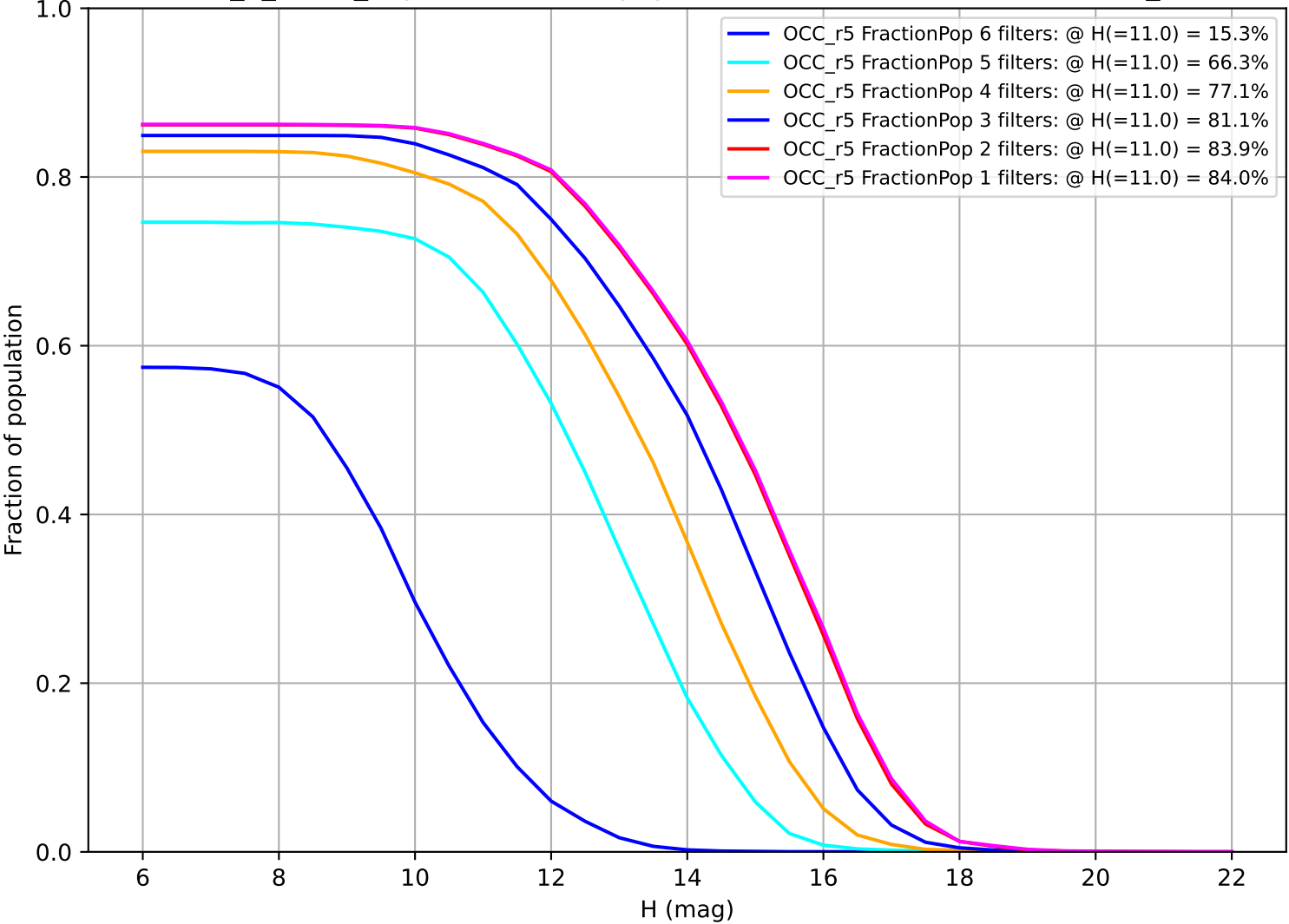
too_5_4v3.4_10yrs: Fraction of population with colors in X filters OCC_r5
