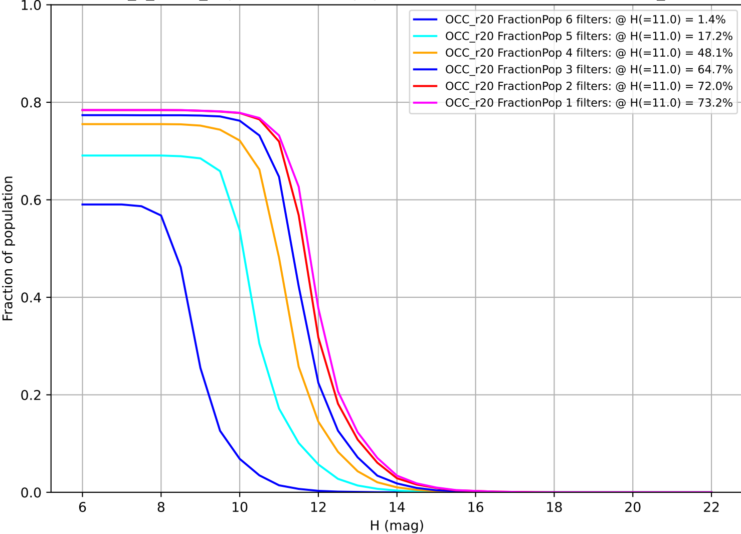
too_5_4v3.4_10yrs: Fraction of population with colors in X filters OCC_r20
