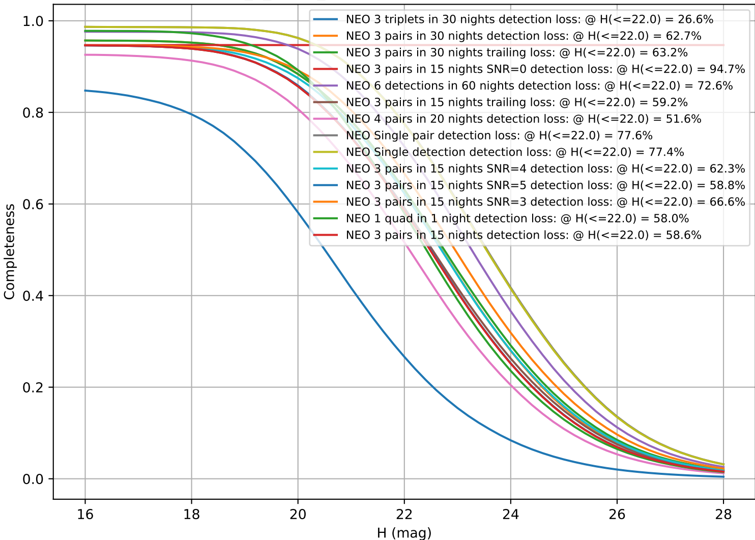
too_5_4v3.4_10yrs: CumulativeCompleteness
