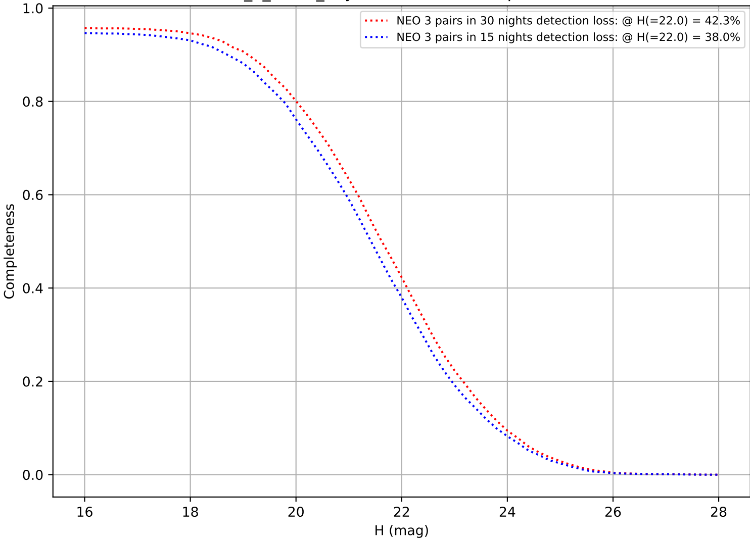
too_5_4v3.4_10yrs: DifferentialCompleteness
