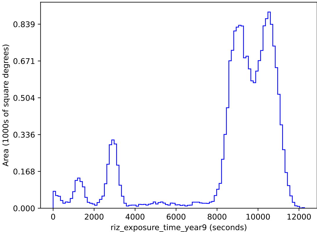
too_5_4v3.4_10yrs gri band non-DD: riz_exposure_time_year9
