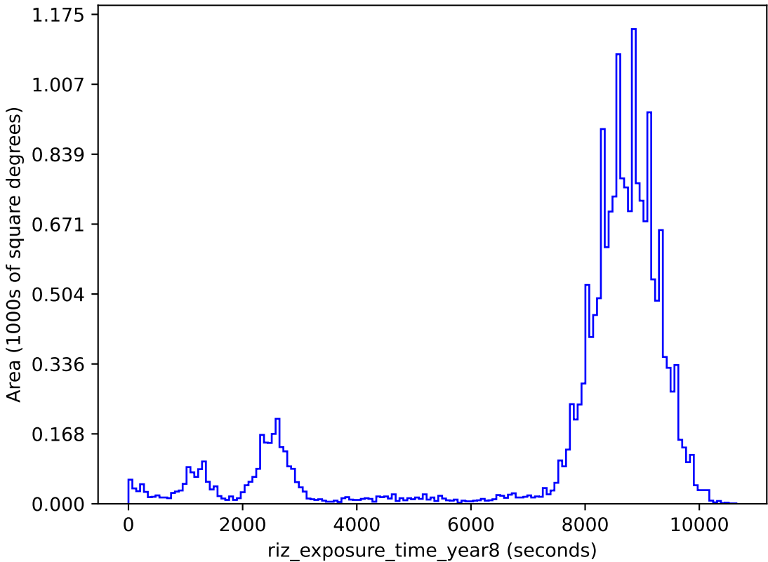
too_5_4v3.4_10yrs gri band non-DD: riz_exposure_time_year8
