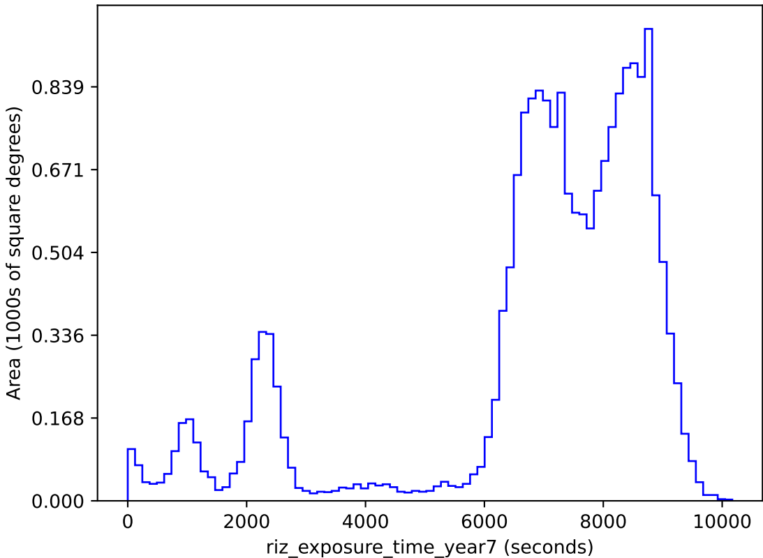
too_5_4v3.4_10yrs gri band non-DD: riz_exposure_time_year7
