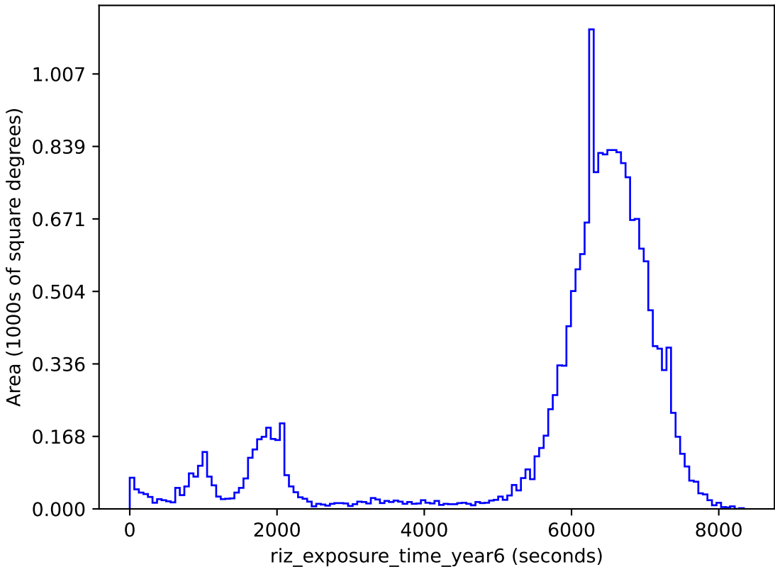
too_5_4v3.4_10yrs gri band non-DD: riz_exposure_time_year6
