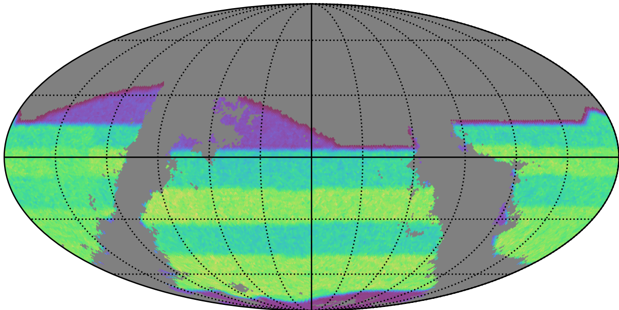
too_5_4v3.4_10yrs gri band non-DD: riz_exposure_time_year5
