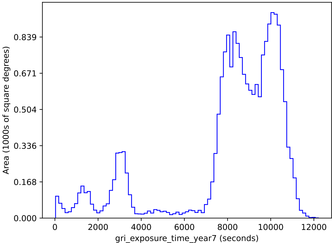
too_5_4v3.4_10yrs gri band non-DD: gri_exposure_time_year7
