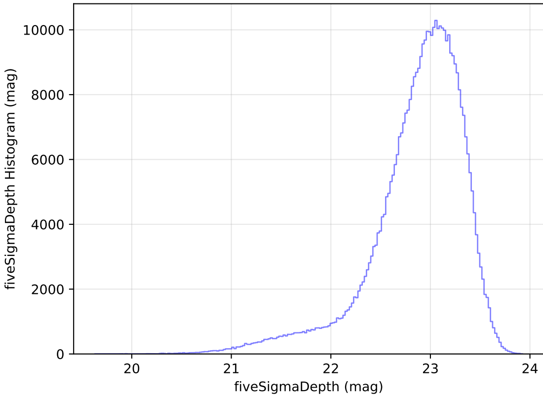
too_5_4v3.4_10yrs z: fiveSigmaDepth Histogram
