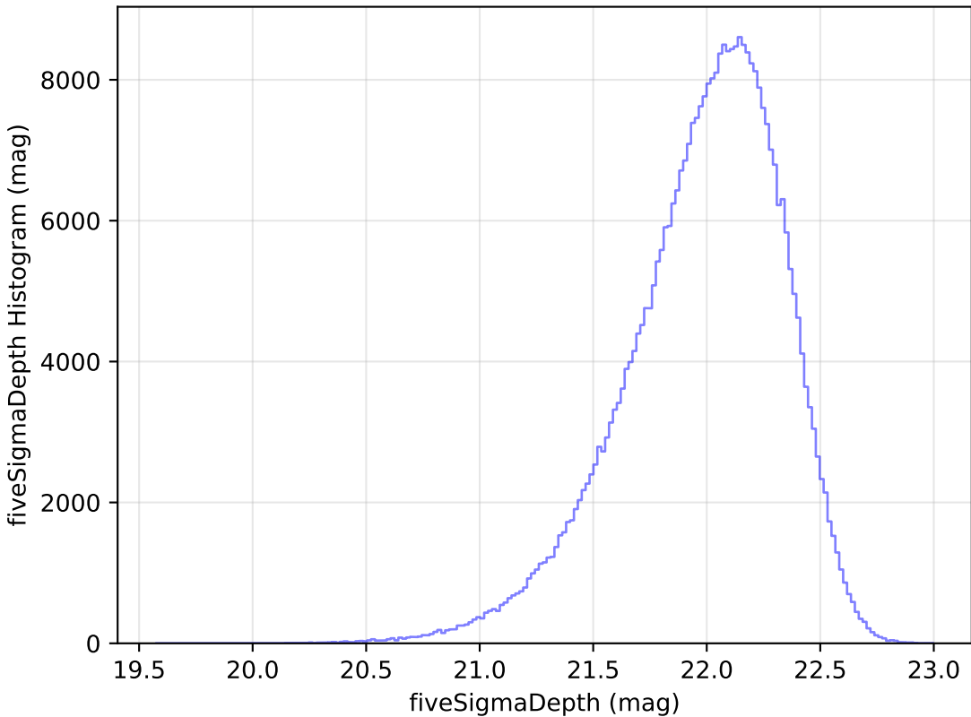
too_5_4v3.4_10yrs y: fiveSigmaDepth Histogram
