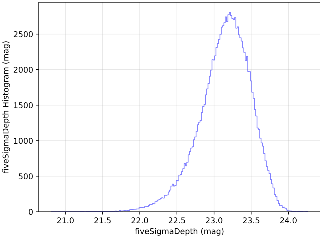
too_5_4v3.4_10yrs u: fiveSigmaDepth Histogram
