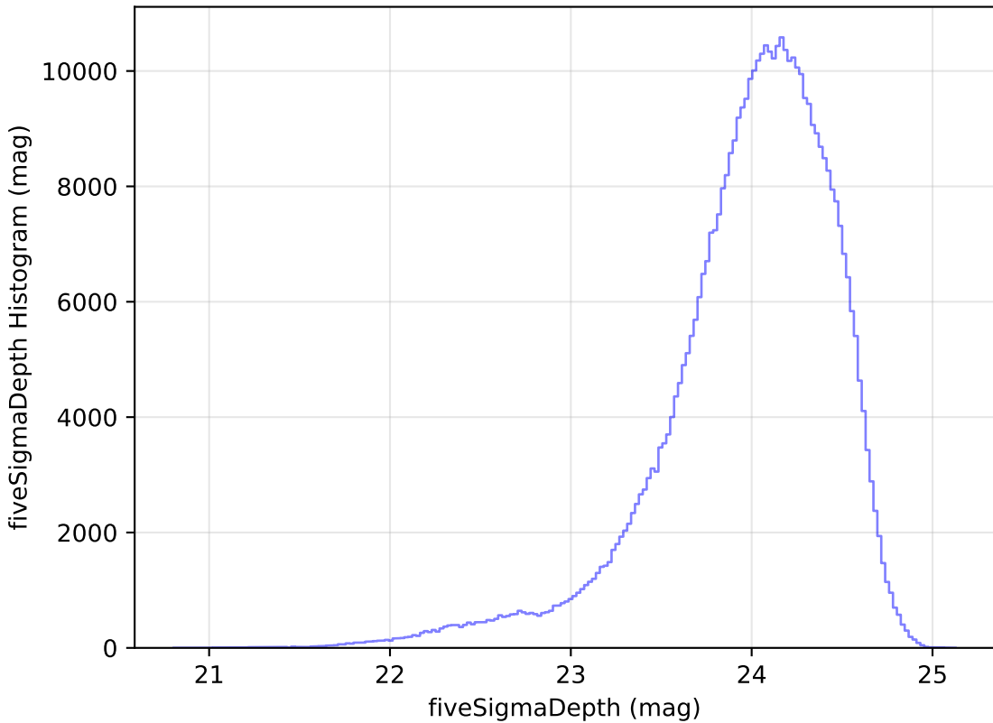
too_5_4v3.4_10yrs r: fiveSigmaDepth Histogram
