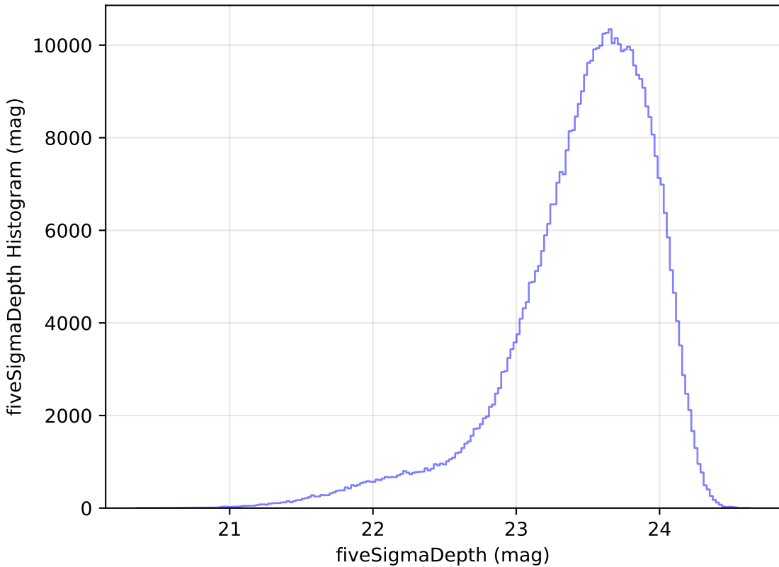
too_5_4v3.4_10yrs i: fiveSigmaDepth Histogram
