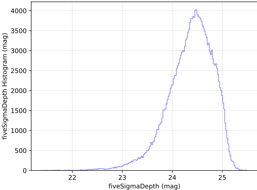
too_5_4v3.4_10yrs g: fiveSigmaDepth Histogram
