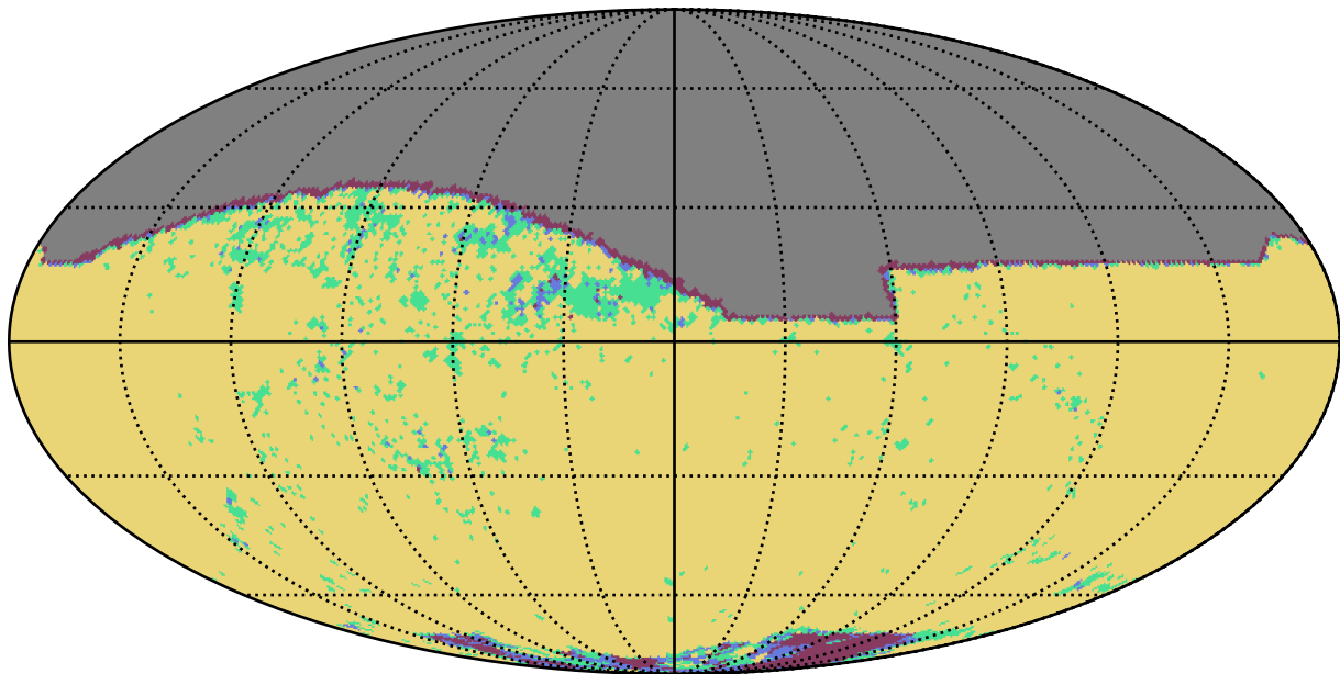
too_5_4v3.4_10yrs z band: YearCoverage night
