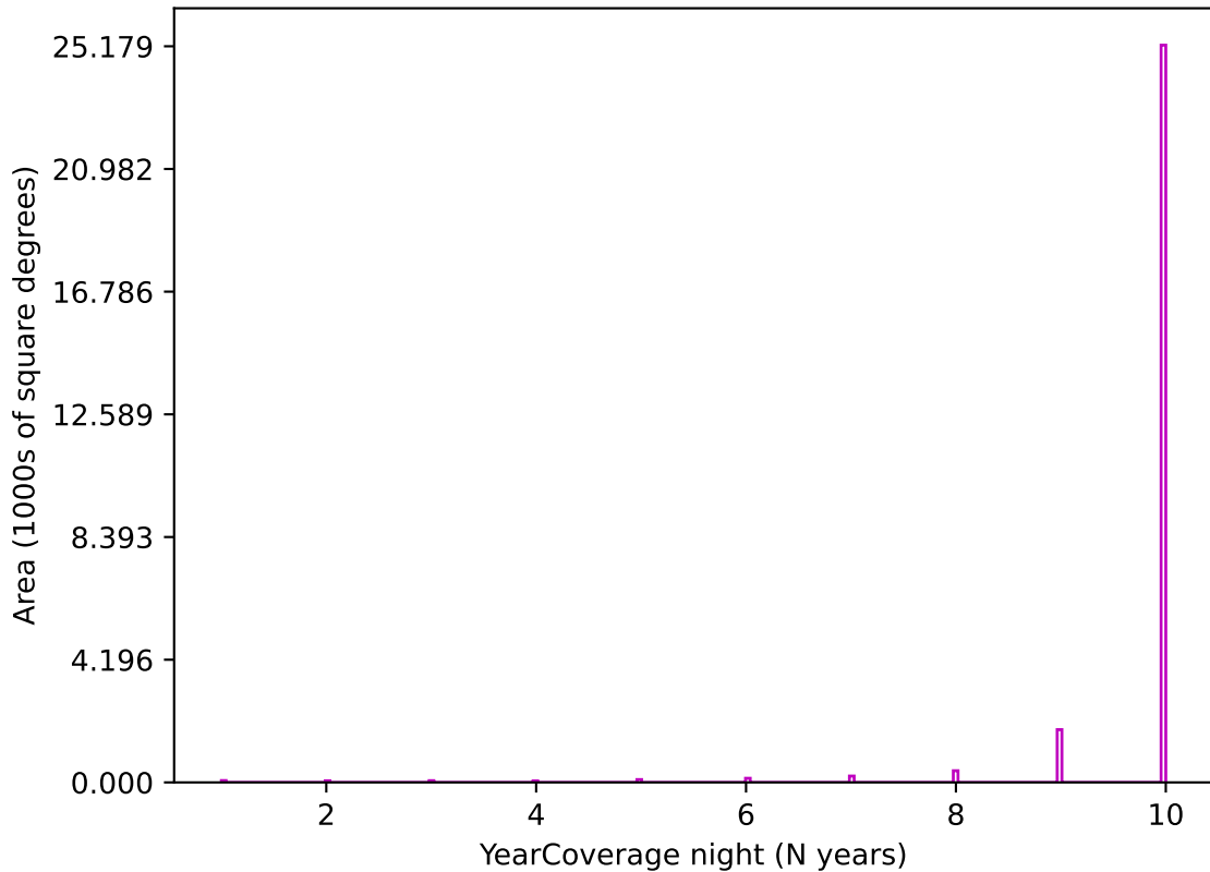
too_5_4v3.4_10yrs z band: YearCoverage night
