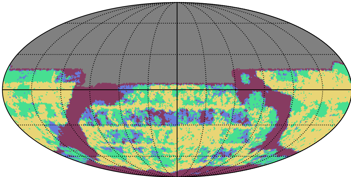
too_5_4v3.4_10yrs u band: YearCoverage night
