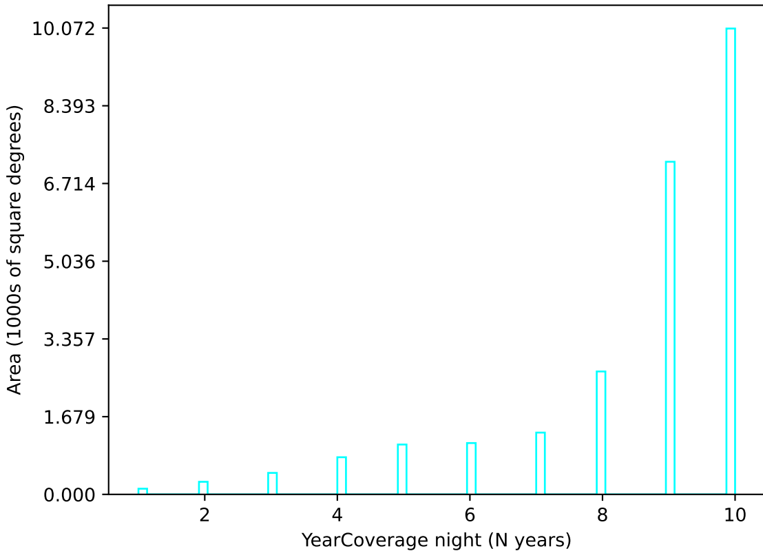
too_5_4v3.4_10yrs u band: YearCoverage night
