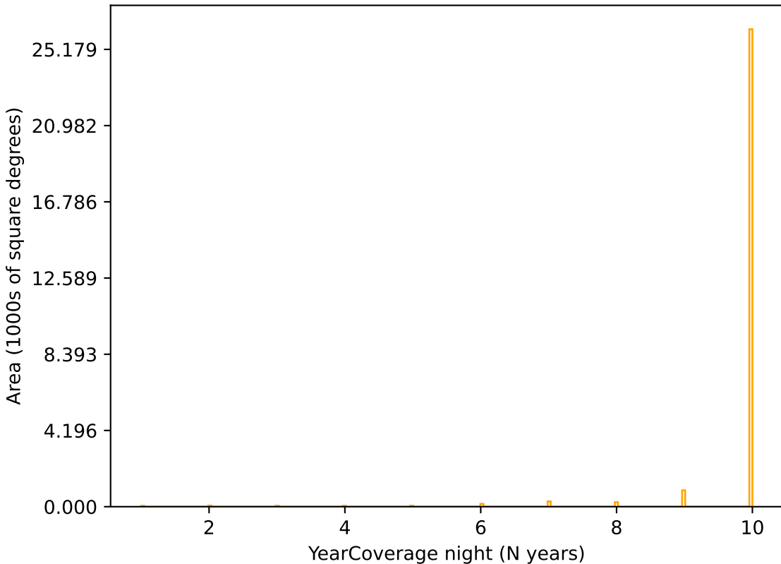
too_5_4v3.4_10yrs r band: YearCoverage night
