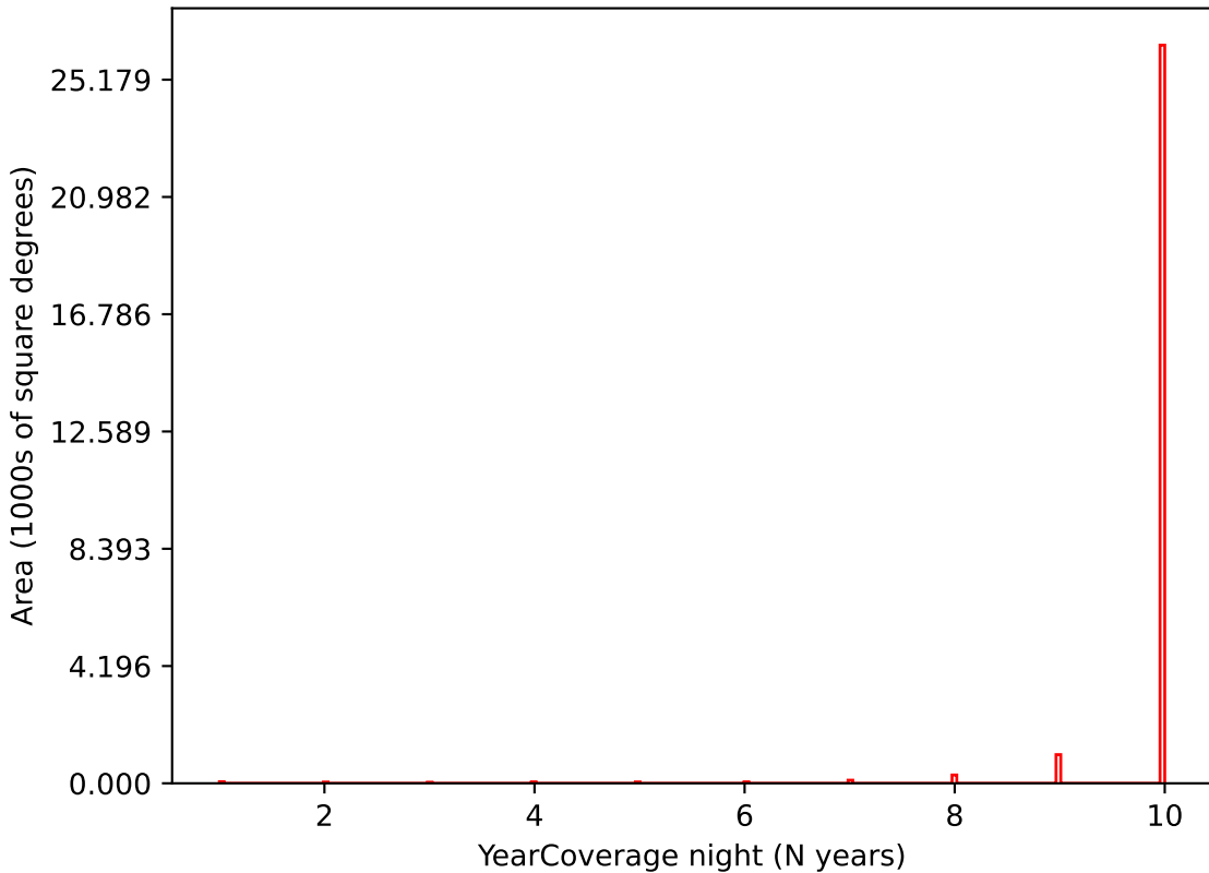
too_5_4v3.4_10yrs i band: YearCoverage night
