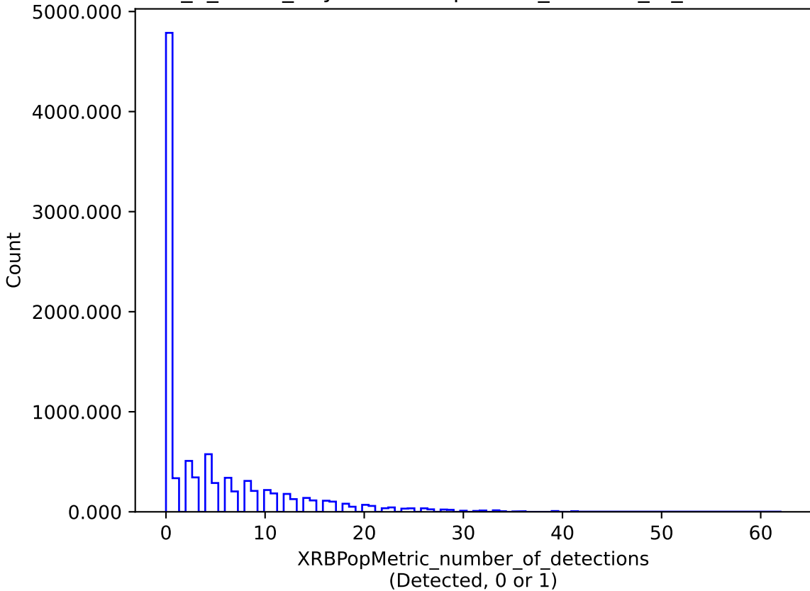
too_5_4v3.4_10yrs : XRBPoMetric_number_of_detections
