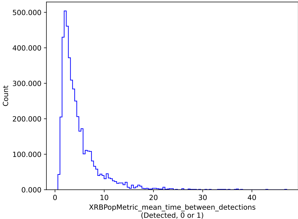
too_5_4v3.4_10yrs : XRBPoMetric_mean_time_between_detections
