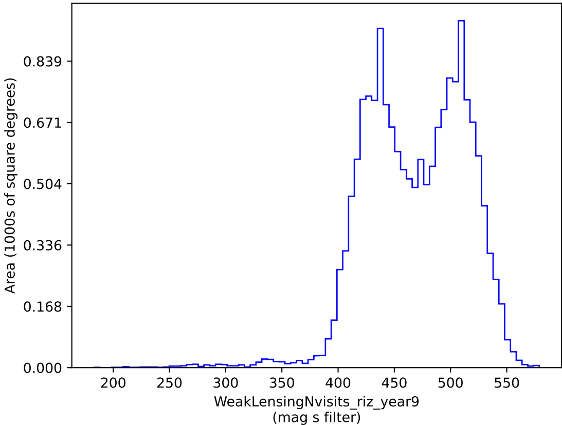
too_5_4v3.4_10yrs gri band non-DD: WeakLensingNvisits_riz_year9
