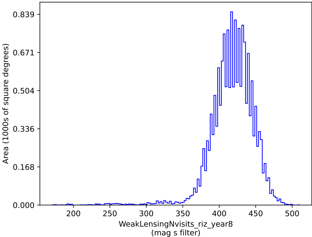
too_5_4v3.4_10yrs gri band non-DD: WeakLensingNvisits_riz_year8
