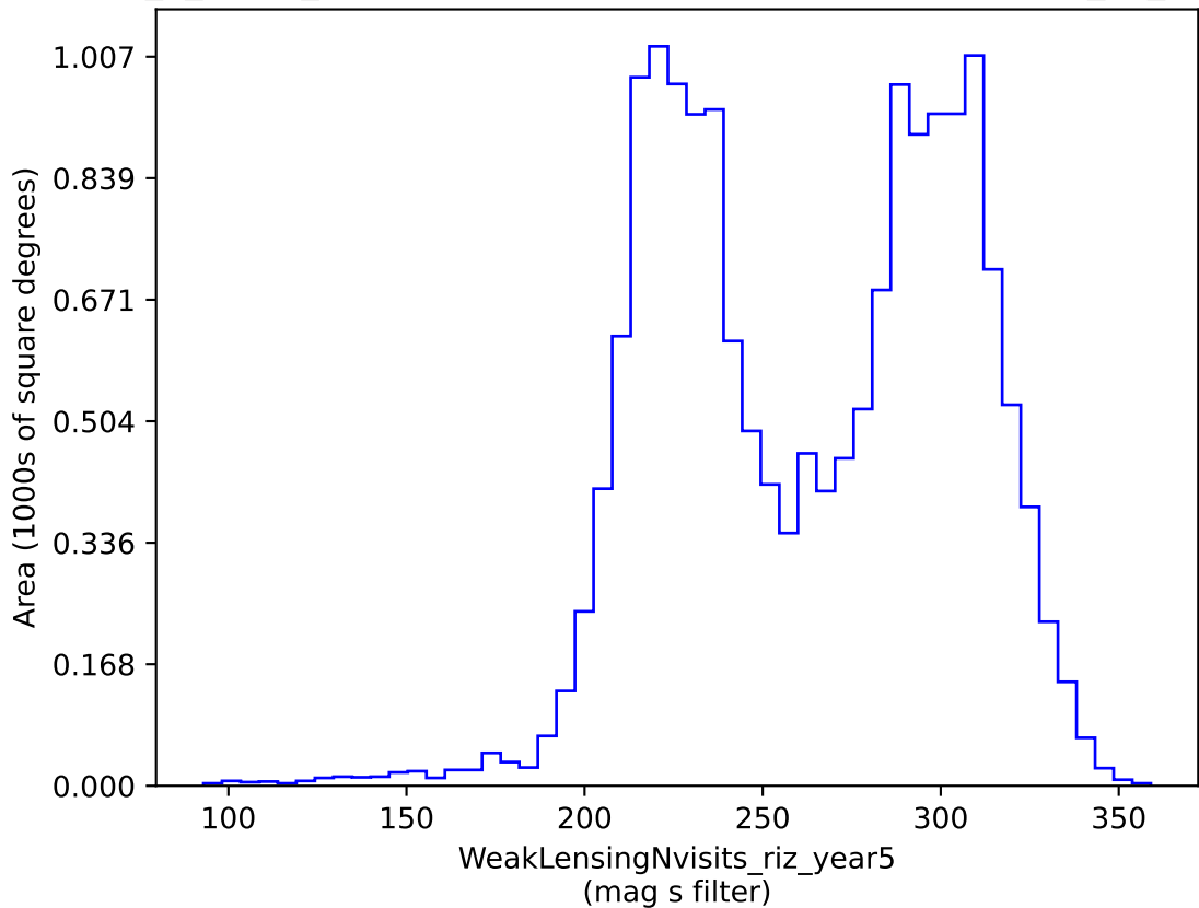
too_5_4v3.4_10yrs gri band non-DD: WeakLensingNvisits_riz_year5
