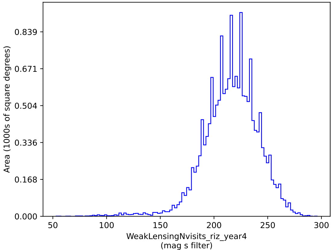
too_5_4v3.4_10yrs gri band non-DD: WeakLensingNvisits_riz_year4
