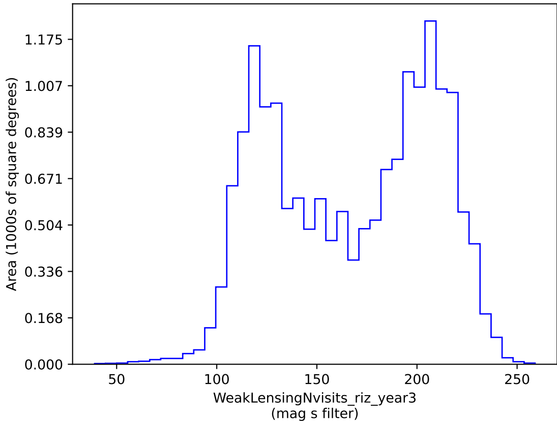
too_5_4v3.4_10yrs gri band non-DD: WeakLensingNvisits_riz_year3
