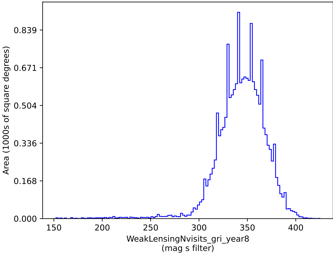
too_5_4v3.4_10yrs gri band non-DD: WeakLensingNvisits_gri_year8
