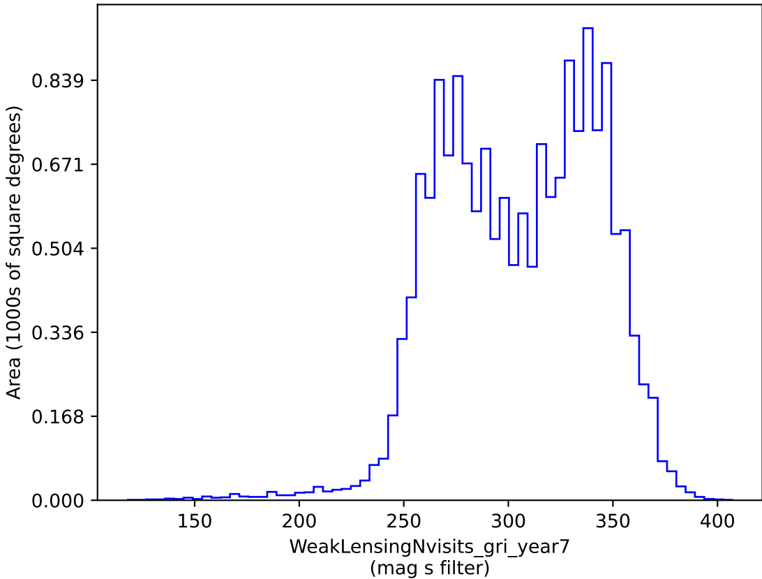
too_5_4v3.4_10yrs gri band non-DD: WeakLensingNvisits_gri_year7
