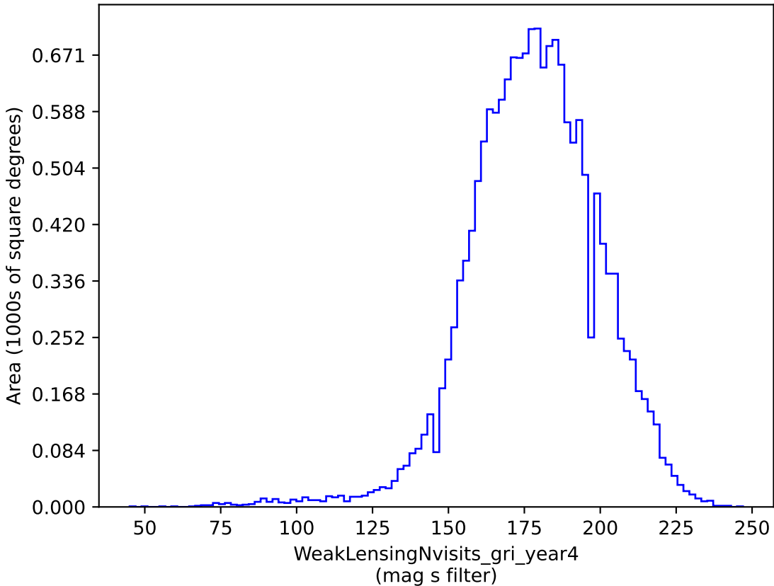
too_5_4v3.4_10yrs gri band non-DD: WeakLensingNvisits_gri_year4
