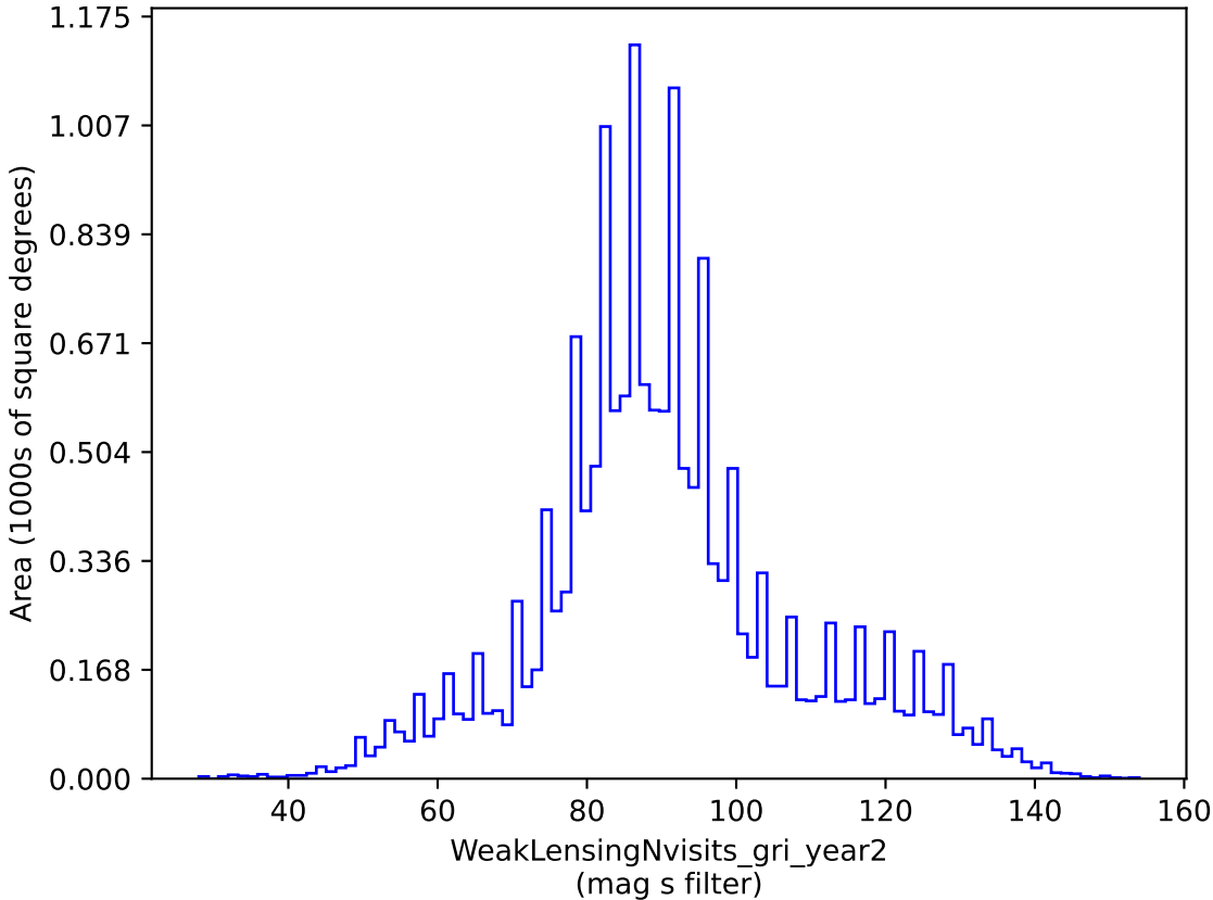
too_5_4v3.4_10yrs gri band non-DD: WeakLensingNvisits_gri_year2
