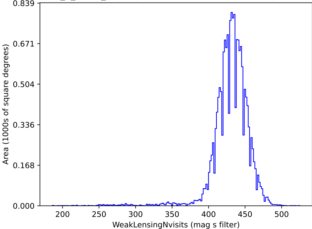
too_5_4v3.4_10yrs gri band non-DD: WeakLensingNvisits
