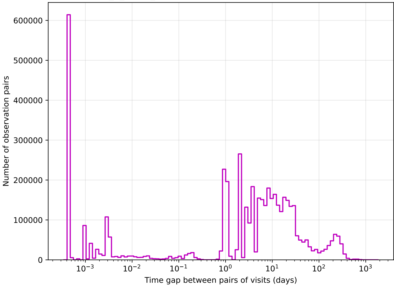
too_5_4v3.4_10yrs z band: Tgaps observationStartMJD
