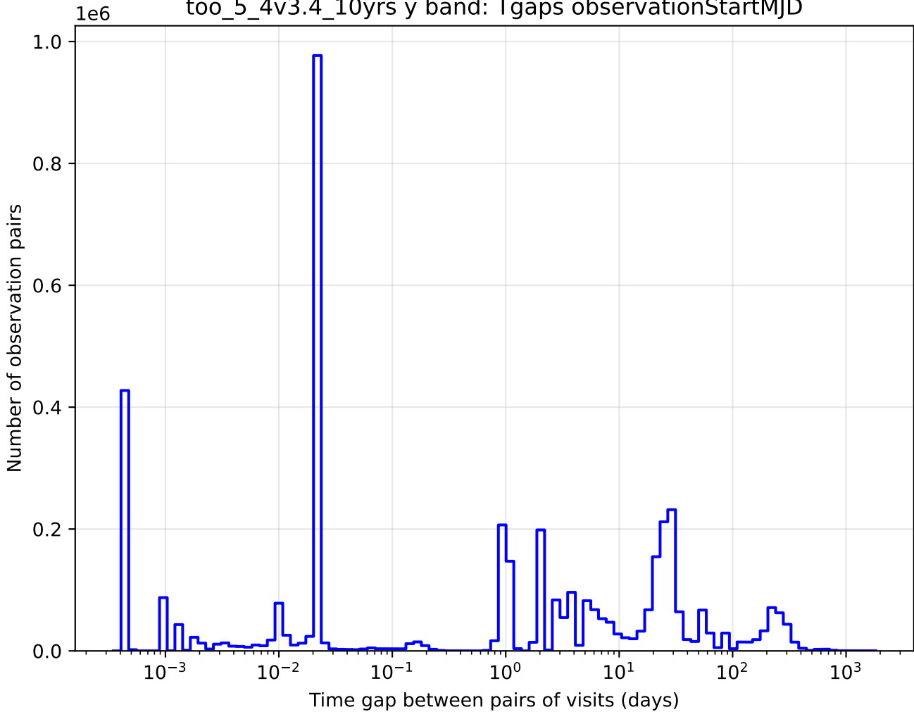
too_5_4v3.4_10yrs y band: Tgaps observationStartMJD
