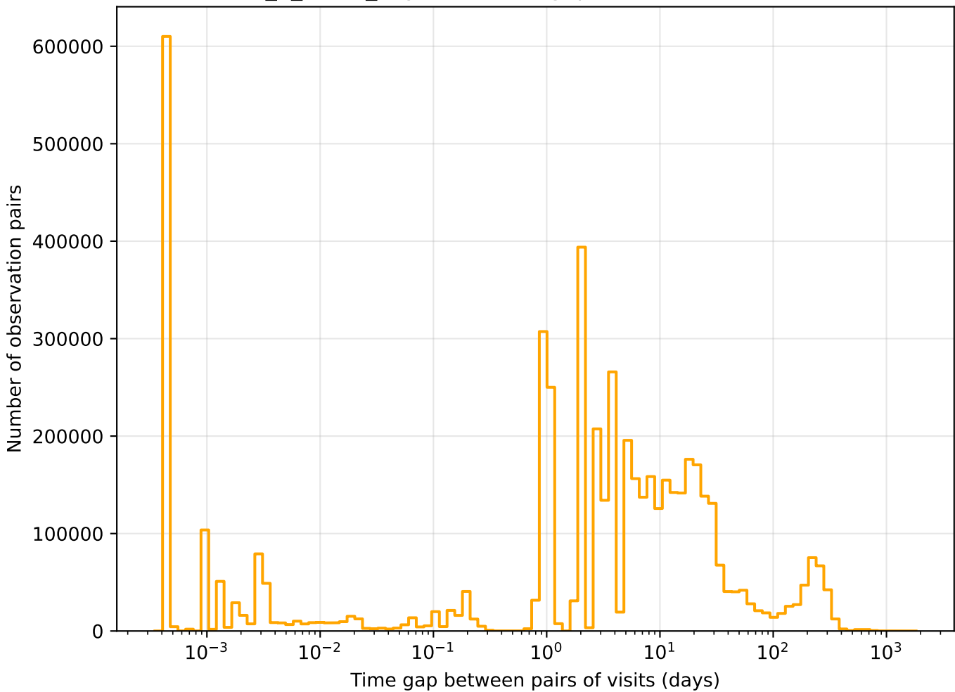
too_5_4v3.4_10yrs r band: Tgaps observationStartMJD
