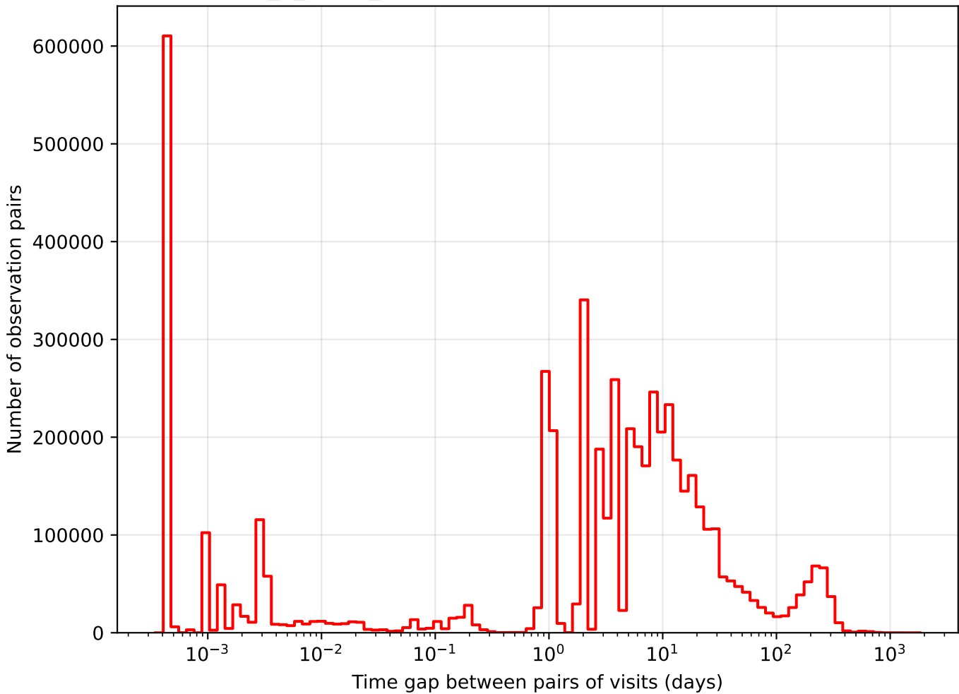
too_5_4v3.4_10yrs i band: Tgaps observationStartMJD
