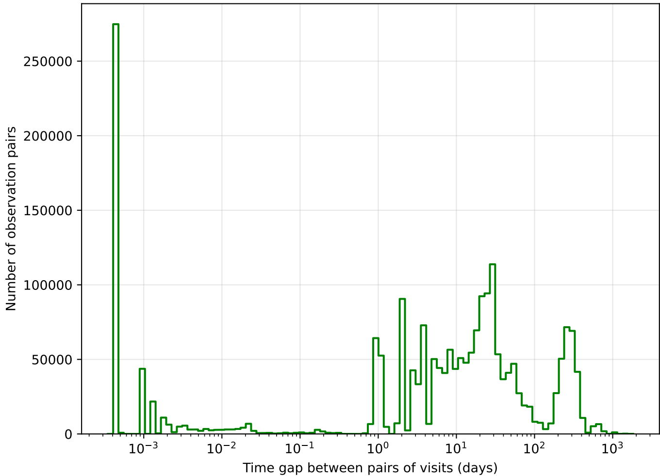
too_5_4v3.4_10yrs g band: Tgaps observationStartMJD
