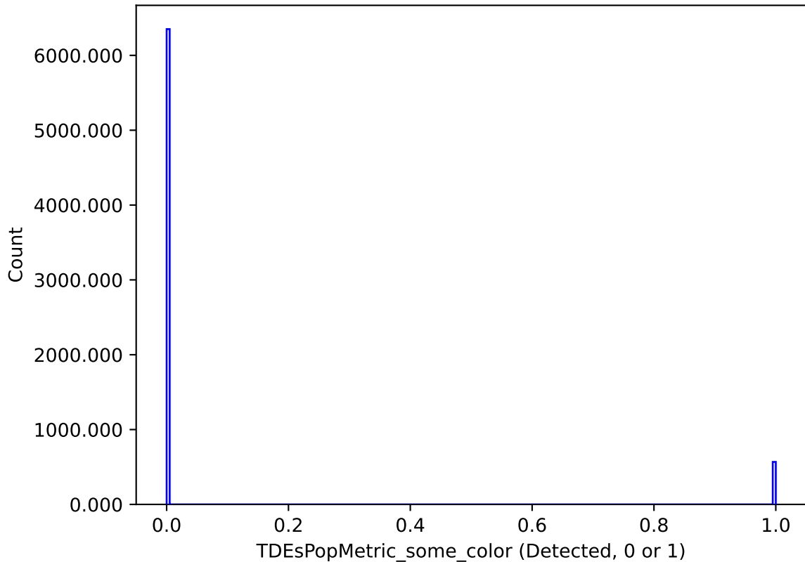
too_5_4v3.4_10yrs : TDEsPopMetric_some_color
