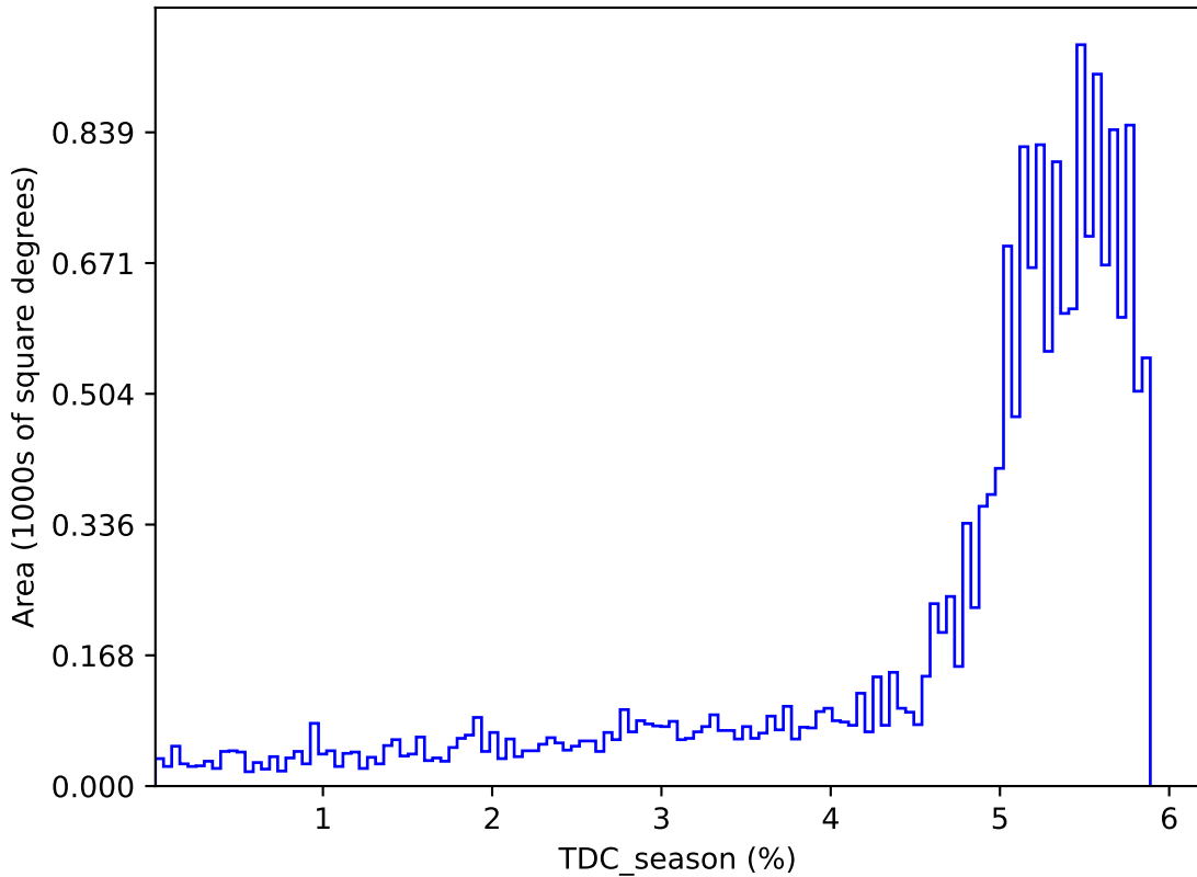
too_5_4v3.4_10yrs : TDC_season
