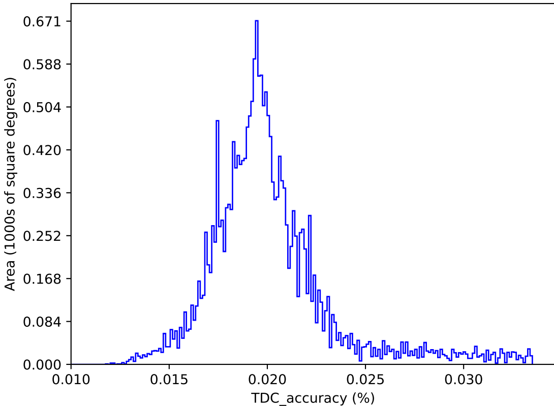
too_5_4v3.4_10yrs : TDC_accuracy
