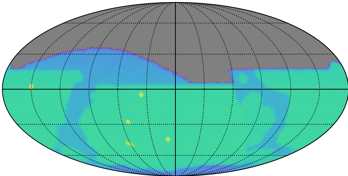
too_5_4v3.4_10yrs z: SurfaceBrightLimit
