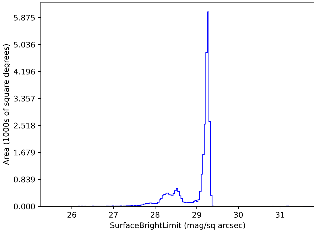
too_5_4v3.4_10yrs z: SurfaceBrightLimit
